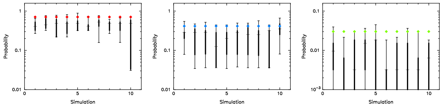
Figure A3. Probability of detecting a magma ocean planet with the ELT 2.2 \mu\text{m} filter in the \beta Pic (left), TW Hydrae (center), and the \eta Cha (right) moving groups, assuming a planetary atmospheric emissivity of \epsilon = 0.01 , using the method in Bonati et al. (2019). The colored diamond symbols indicate the probability of detecting a magma ocean planet around all M-stars, G-stars, and A-stars combined, assuming the numbers of stars presented in recent literature (Gagné et al. 2018a, 2018b). The error bars indicate the full range of detection probabilities from randomly sampling the IMF 10 times, and the thicker portions of the error bars indicate the interquartile range. The median values are shown by the horizontal lines. In each figure panel, the experiment has been repeated 10 times and the original data point from Figure 2 is on the far left of each panel. Note the different y-axis scale in panel (c).
