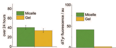
Fig. 5 Comparison of photochemical reactivity in 5 mg mL -1 micelle and gel systems for PEG2000–Tyr 6 . Measured by tyrosine degradation (left) and dityrosine formation (right).
