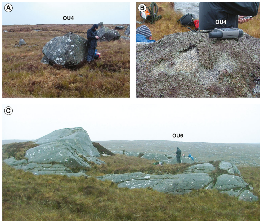
Fig. 5. The Rossaveel region is characterized by glacially scoured terrain with roches moutonnées and glacially sculpted bedrock bumps. Samples were taken from two erratics (OU4 and OU5) and the lee-side of a roche moutonnée (OU6; Tables 1–3). A, B. OU4, an erratic, provided an exposure age of 16.3 \pm 1.8 ka. Note the heavy lichen cover on this sample. C. Sample OU6 was taken from bedrock surface in the lee-side of a large roche moutonnée, which provided an age of 18.4 \pm 1.1 ka. Using only OU04+06 provides an UWM of 18.2 \pm 1.0 ka, but this has a low level of confidence.
