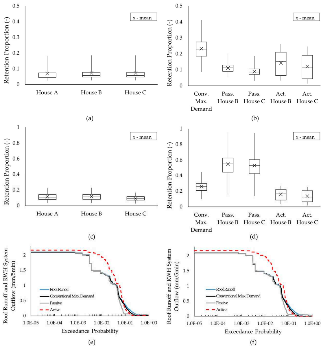
Figure 4. Modelled stormwater management performance during 30 largest events: (a) retention—original demand; (b) retention—suggested scenarios; (c) retention below greenfield runoff—original demand; (d) retention below greenfield runoff—suggested scenarios; (e) flow duration curve—House B; (f) flow duration curve—House C.
