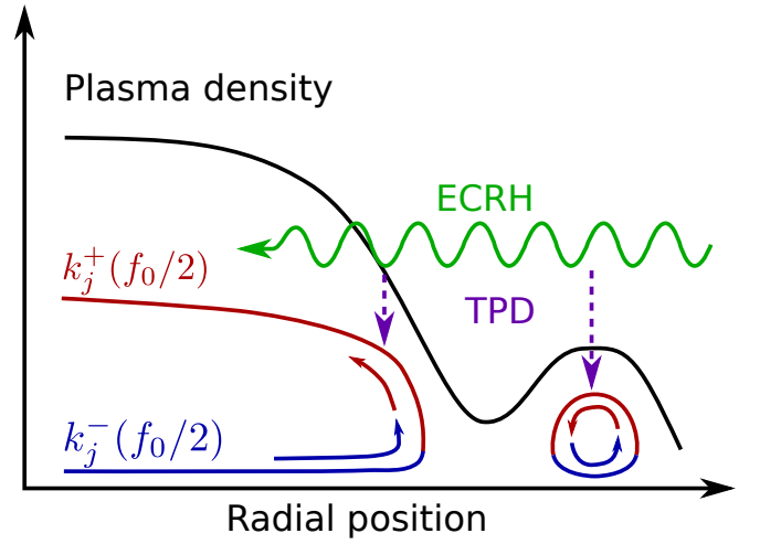
FIG. 2: A sketch showing how a non-monotonic density profile caused by a magnetic island can allow for UH waves to become trapped locally. An ECRH gyrotron beam, aiming for the plasma core, may decay through TPD near the 2nd harmonic UH layer and excite two trapped half frequency waves inside the island. Linear conversion between X-mode and EBWs at the UH layer is the trapping mechanism. In the plasma core, waves can be convected away from the decay region.
