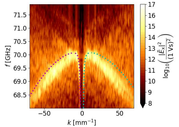
(c) FFT for -5 \text{ mm} < x < 5 \text{ mm} and the time interval 50 \text{ ns} < t < 60 \text{ ns} , corresponding to phase C in figure 6a. The added dotted magenta line is the dispersion relation at the then elevated mean electron temperature of 120 eV.
