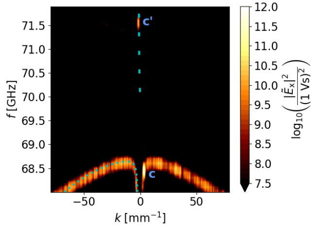
(b) k - and f -space for 55 \text{ ns} < t < 65 \text{ ns} with the profile shown in figure 8a and an intensity of I_{\text{pump}} = 10 \text{ kW/mm}^2 ; one trapped, c , and one escaping wave, c' , are excited. The dotted cyan line in the lower half shows dispersion lines for trapped wave in negative k , equation (3), while the more spaced out dotted line in the top half indicates escaping X-mode waves in negative k , equation (2). This spectrum is not directly comparable to figure 7c due to a change in both density and pump intensity.
