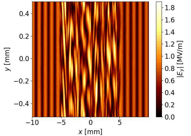
(b) A snapshot of the y -component of the electric field at t = 30 ns, after the primary daughter waves have visibly formed. Note that the scales on the x - and y -axes are not the same. Unlike the pump wave, the trapped waves not only propagate in the x -direction. Compare to the 1D figure in figure 6a.
