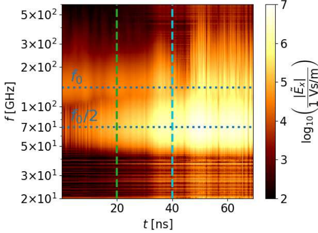
(b) A CWT of figure 6a at the x = 0 mm center line. Dotted horizontal blue lines mark frequencies as labeled above them. Dashed vertical lines indicate phases as shown by corresponding colors in figure 6a.
