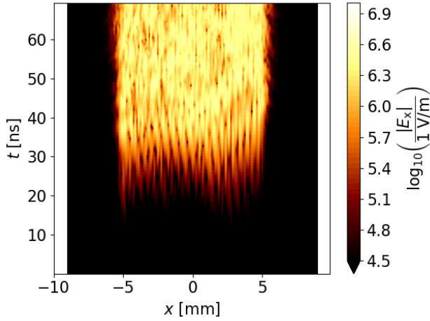
(a) Evolution of the longitudinal electric field for immobile ions in time and space, compare with figure 6a where plasma parameters are the same but ions are mobile.
