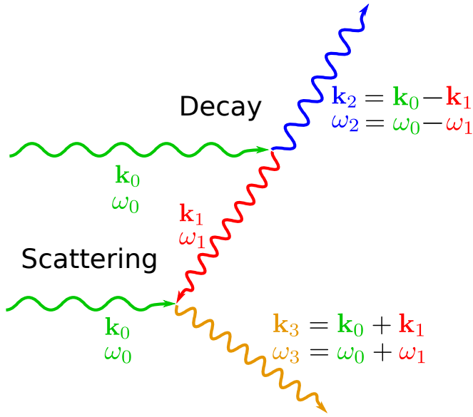
FIG. 1: An illustration of two types of PIs involving three waves: a decay into two waves, and scattering or combination of two waves. Both satisfy equations (1). As indicated, a long wavelength wave may decay into two short wavelength waves provided that their k -vectors point in different directions; such would be the typical situation for TPD.
