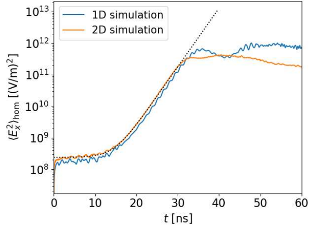
(a) Mean squared x -component of the electric field averaged over the homogeneous center of the 2D domain for a simulation with a pump intensity of I_{\text{pump}} = 1 kW/mm 2 . The mean squared field is compared to a 1D simulation of similar parameters and the growth of the 2D simulations is fitted with an exponential function. The
