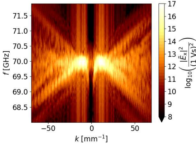
(b) k - and f -space for 50 \text{ ns} < t < 60 \text{ ns} , compare with figure 7c where plasma parameters are the same but ions are mobile.
