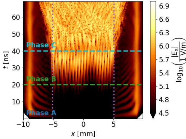
(a) Longitudinal electric field component in time and space. Colored dashed horizontal lines mark the beginning of the phase as labeled above it, used for reference in the text. Dotted vertical purple lines mark the UH layer for 70 GHz UH waves. The slow oscillations outside the homogeneous region are ion waves, see the text.
