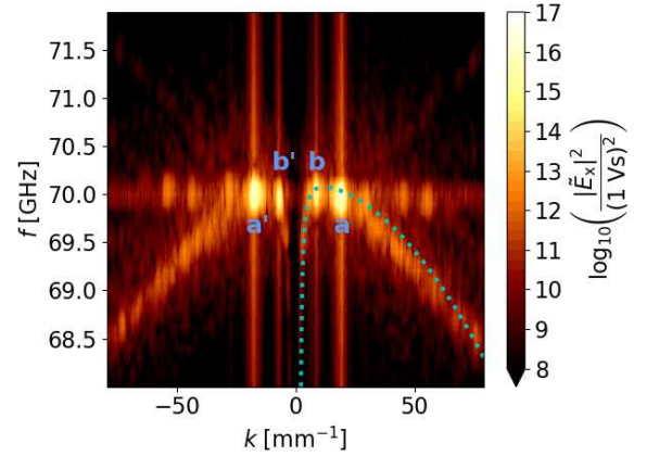
(b) FFT for -5 \text{ mm} < x < 5 \text{ mm} and the time interval 25 \text{ ns} < t < 35 \text{ ns} , corresponding to phase B in figure 6a.
