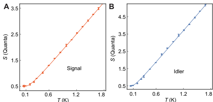
Fig. 5. System noise calibration. Calibration of signal (A) and idler (B) output channels. The measured noise density in units of quanta, S_i = N_i / (\hbar\omega_i BRG_i) - n_{add,ir} is shown as a function of the temperature T of the 50-ohm load. The error bars indicate the SD obtained from three measurements with 576,000 quadrature pairs each. The solid lines are fits to Eq. 5 in units of quanta, which yields the system gain and noise with the standard errors (95% confidence interval) as stated in section Results.
