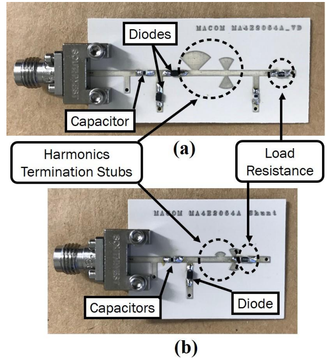
FIGURE 10: Fabricated rectifier circuits a) voltage-doubler, b) shunt.
