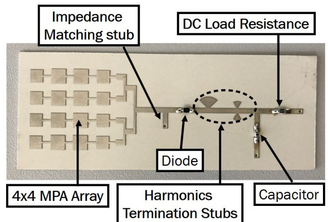
FIGURE 13: Fabricated rectenna sample.
