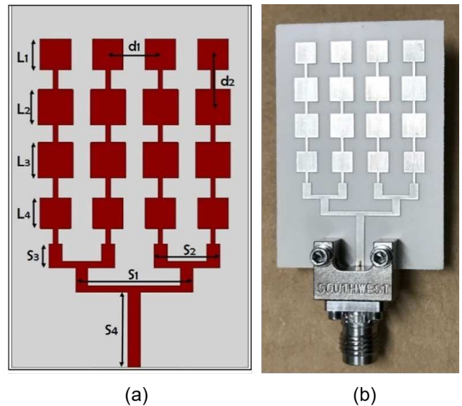
FIGURE 7: Planar 4x4 MPA array, a). Array layout with dimensions L1=L4=3.5 mm, L2=L3=4 mm, d1=d2=6 mm, S1=13.4 mm, S2=7.5 mm, S3=2.7 mm, S4=8.55 mm, b). Fabricated array.
