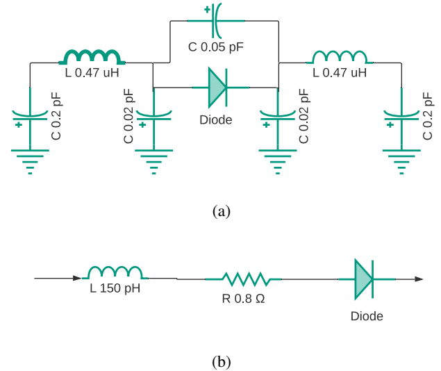
FIGURE 2: Diode package model a) SOD-323, b) 0201.
