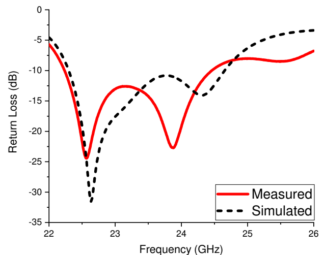
FIGURE 8: Simulated and measured return loss performance.
