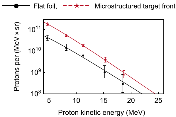
FIG. 3. Combined proton spectra derived from radiochromic film stacks together with the approximated Maxwell distribution. Error bars indicate the standard deviation.
