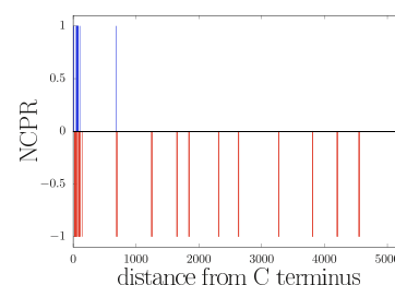
Figure 1. Net charge per residue (NCP) of the silk protein (sequence under ref 19) as determined using localCIDER. 20
