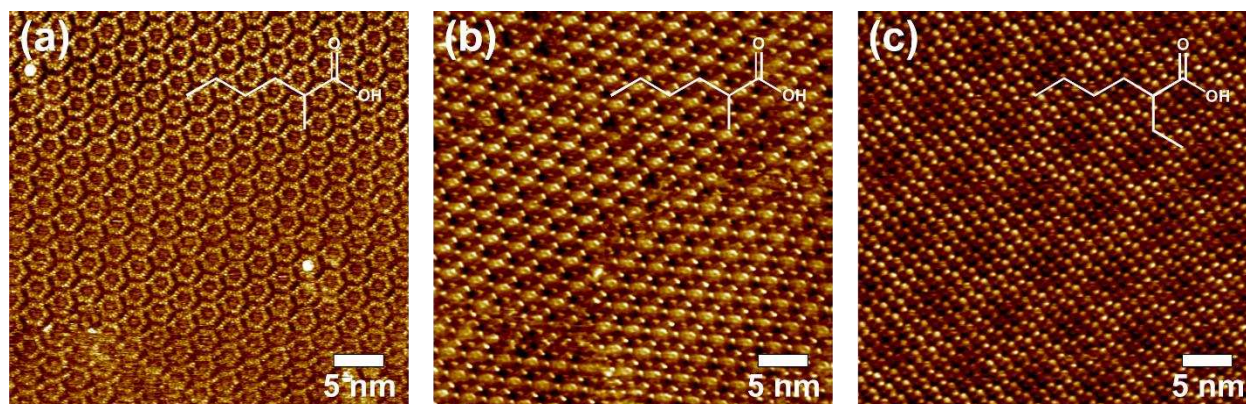
Figure 4. STM images of TMA monolayers on graphite(0001) acquired in saturated solutions using (a) / (b) methyl-6A and (c) ethyl-6A as solvent. Overlays show chemical structures of respective solvents. While methyl-6A still results in the flower polymorph, the chickenwire polymorph is observed in ethyl-6A. (sample voltages and current setpoints: (a) -582 mV, 61 pA; (b) -582 mV, 54 pA; (c) -571 mV, 54 pA).
