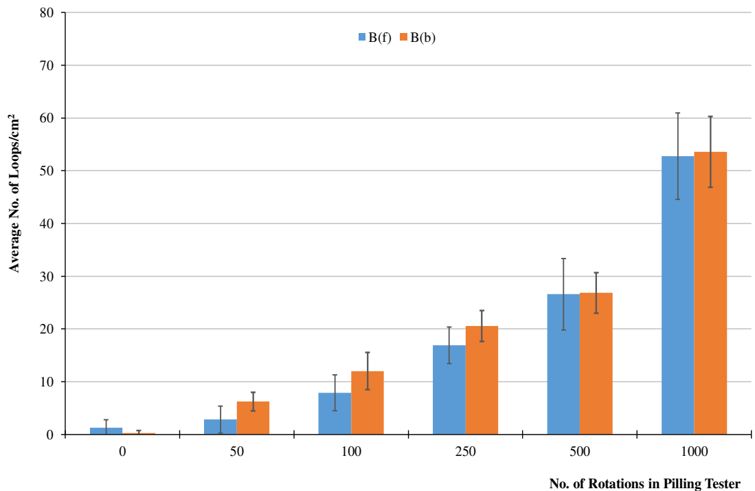
Figure 12. Average loop formation per cm 2 developed after a known number of rotations of Specimen B within the Pilling Box tester
