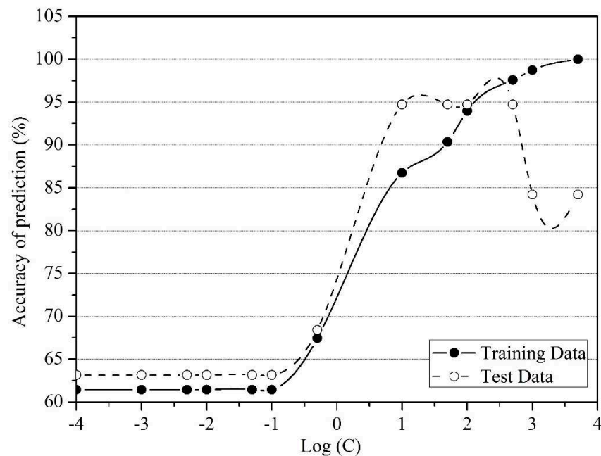
Figure 7. Dependence of the accuracy of classification on the cost parameter C .
