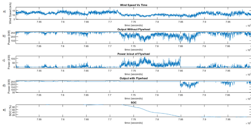
Fig. 6. Operation of simulation during period of breaching export limit (a) Wind Speed (b) Output to grid without FESS (c) Power in/out of FESS (d) Output to grid with FESS (e) State of charge of FESS.
