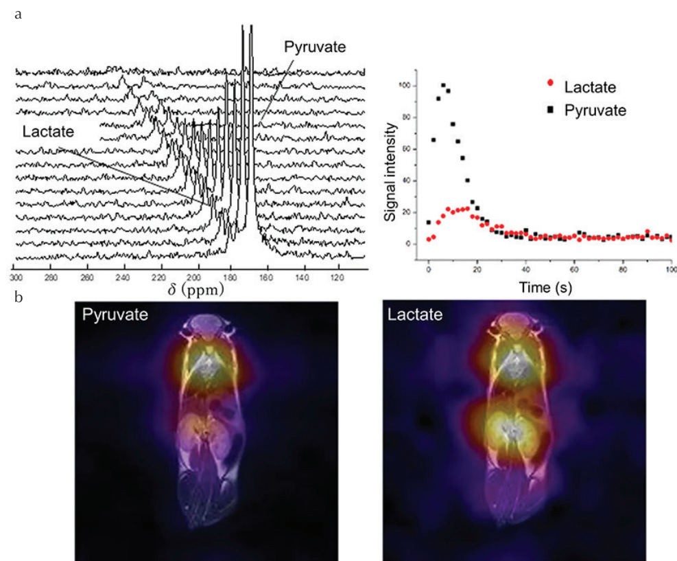
Fig. 7 (a) Slice-selective dynamic ^{13}\text{C} MRS of a healthy wild-type mouse after injection of HP [1-^{13}\text{C}] pyruvate produced by parahydrogen-induced polarization (PHIP)-side-arm hydrogenation (SAH), and (b) corresponding whole-body ^{13}\text{C} chemical shift imaging (CSI) of [1-^{13}\text{C}] pyruvate and [1-^{13}\text{C}] lactate (reproduced from Figs. 2 and 3 of Cavallari et al. 145 under the Creative Commons CCBY License).
