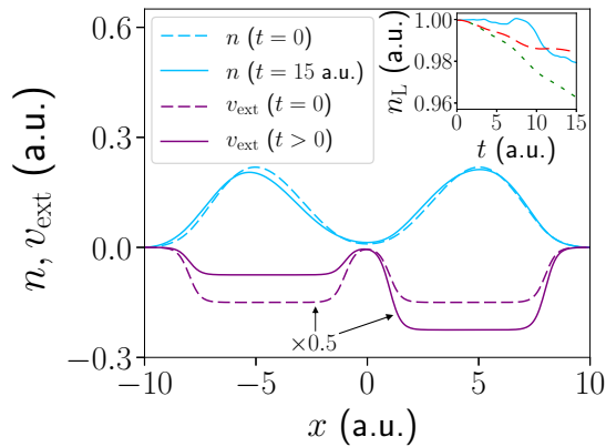
FIG. 4. System 3: Two interacting electrons in a tunneling system. Inset: The exact total electron number on the left-hand side ( x < 0 ) (short-dashed green); also the exact adiabatic (solid blue) and fluidic approximation (dashed red).
