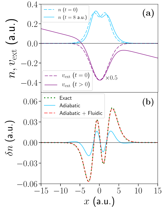
FIG. 1. System 1: Two interacting electrons in a Gaussian potential well, with a uniform electric field applied at t = 0 , driving the electrons to the right and inducing a current. (a) The ground-state external potential (dashed purple) and exact ground-state electron density (dashed blue), along with the perturbed external potential (solid purple) and exact time-dependent electron density at t = 8 a.u. (solid blue). (b) The change in the exact electron density [ \delta n(x, t) = n(x, t) - n(x, 0) ] at t = 8 a.u. (short-dashed green), along with that obtained when using the exact v_{\text{KS}}^{\text{A}} (solid blue), and when adding the exact v_{\text{KS}}^{\text{A}} with the fluidic approximation \Delta A_{\text{KS}} = -u (dashed red). The exact adiabatic potential is clearly inadequate, but its error is substantially reduced by the fluidic approximation.
