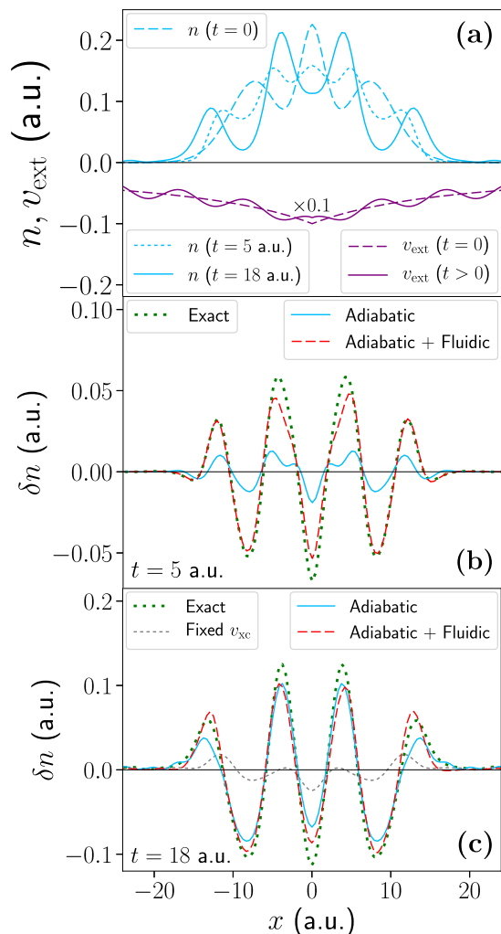
FIG. 3. System 2C: Three interacting electrons in an atomiclike potential, with a static sinusoidal perturbation applied at t = 0 , pushing the electrons apart. (a) The ground-state external potential (dashed purple) and exact ground-state electron density (dashed blue), along with the perturbed external potential (solid purple) and exact time-dependent electron density at t = 5 a.u. (short-dashed blue) and t = 18 a.u. (solid blue). (b) The change in the exact electron density at t = 5 a.u. (short-dashed green), along with that obtained when using the exact v_{KS}^A (solid blue), and when adding the exact v_{KS}^A with the fluidic approximation (dashed red). Even though the density is strongly disrupted, the fluidic approximation remains successful. (c) The same as (b) but at t = 18 a.u., where the dynamic xc contribution is very significant, evident by the completely inadequate result obtained with the fixed v_{xc} (short-dashed gray) (see main text). Here, the exact v_{KS}^A is better, but adding the fluidic approximation improves it further.
