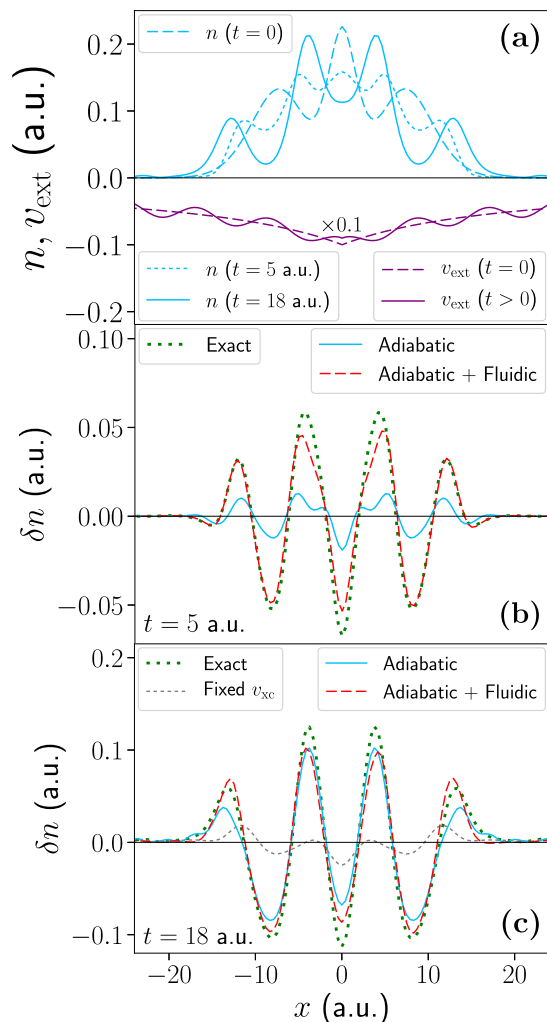
FIG. 3. System 2C: Three interacting electrons in an atomiclike potential, with a static sinusoidal perturbation applied at t = 0 , pushing the electrons apart. (a) The ground-state external potential (dashed purple) and exact ground-state electron density (dashed blue), along with the perturbed external potential (solid purple) and exact time-dependent electron density at t = 5 a.u. (short-dashed blue) and t = 18 a.u. (solid blue). (b) The change in the exact electron density at t = 5 a.u. (short-dashed green), along with that obtained when using the exact v_{KS}^A (solid blue), and when adding the exact v_{KS}^A with the fluidic approximation (dashed red). Even though the density is strongly disrupted, the fluidic approximation remains successful. (c) The same as (b) but at t = 18 a.u., where the dynamic xc contribution is very significant, evident by the completely inadequate result obtained with the fixed v_{xc} (short-dashed gray) (see main text). Here, the exact v_{KS}^A is better, but adding the fluidic approximation improves it further.
