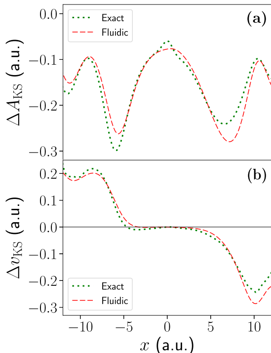
FIG. 2. The nonadiabatic correction to the KS potentials for system 1. (a) The exact \Delta A_{KS} (short-dashed green) and that obtained using the fluidic approximation \Delta A_{KS} = -u (dashed red), at t = 8 a.u. (b) The corresponding exact (short-dashed green) and fluidic (dashed red) \Delta v_{KS} in its scalar form. The fluidic approximation performs very well, even though the velocity field is non-uniform in both space and time. (The exact adiabatic approximation, of course, amounts to setting \Delta A_{KS} = \Delta v_{KS} = 0 )
