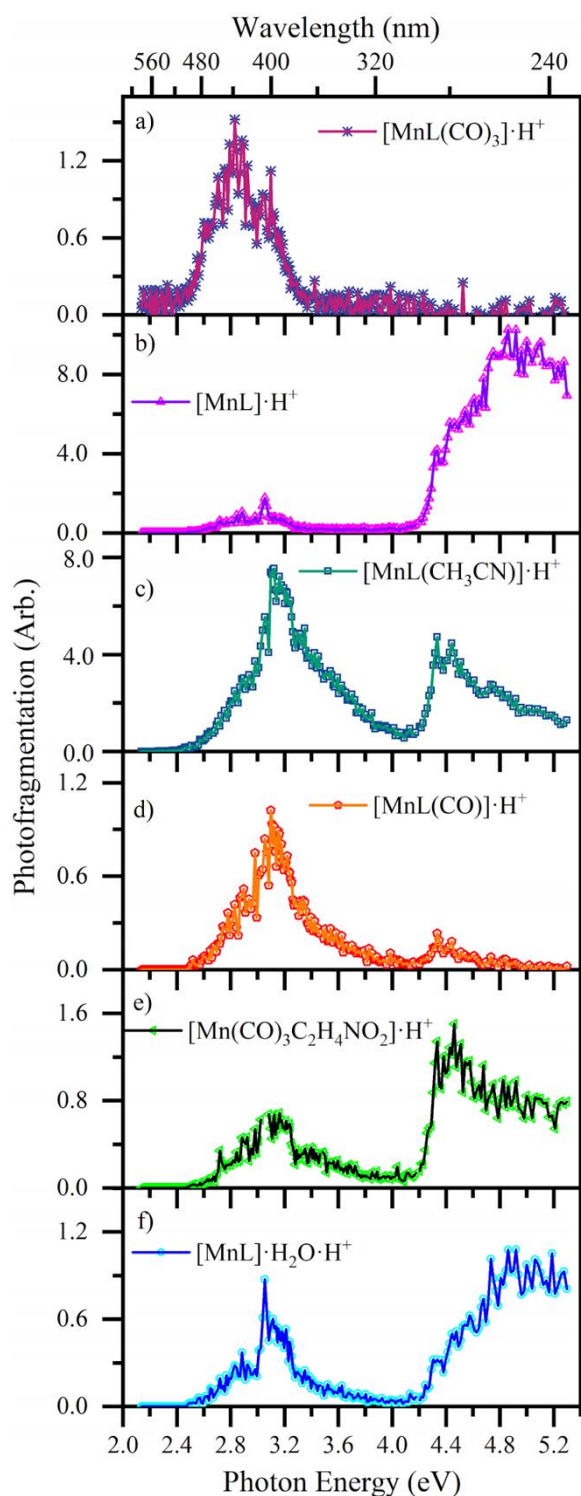
Figure 6. Photofragment production spectra from [\text{MnL}(\text{CO})_3(\text{CH}_3\text{CN})]\cdot\text{H}^+ across the range 2.1-5.3 eV, showing production of (a) [\text{MnL}(\text{CO})_3]\cdot\text{H}^+ , (b)
