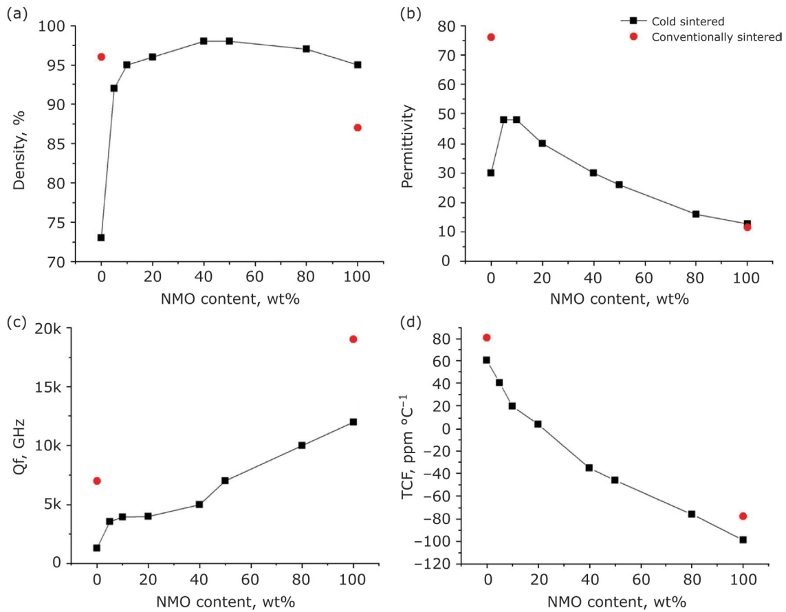
Fig. 6. (a) Density; (b) permittivity; (c) Qf ; and (d) TCF of cold sintered BLVMO-NMO composite ceramics and conventionally sintered BLVMO and NMO. Adapted from (19) under Creative Commons Attribution 4.0 International (CC BY 4.0)
