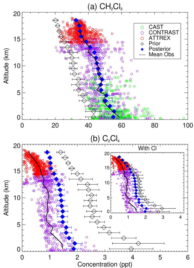
Figure 8. Modeled versus observed vertical profiles of (a) \text{CH}_2\text{Cl}_2 and (b) \text{C}_2\text{Cl}_4 volume mixing ratio (ppt) during the 2014 CAST/CONTRAST/ATTREX field missions in the West Pacific (see section 3.2). Model output has been averaged in 1 km vertical bins and is shown for both the prior and posterior emissions. Note that these aircraft data are “independent” in that they were not used in the inversion to produce the posterior emissions. The \text{C}_2\text{Cl}_4 + \text{Cl} sink data are inset in (b). For \text{CH}_2\text{Cl}_2 , results are generated using the posterior emissions from the no ocean inversion scenario.
