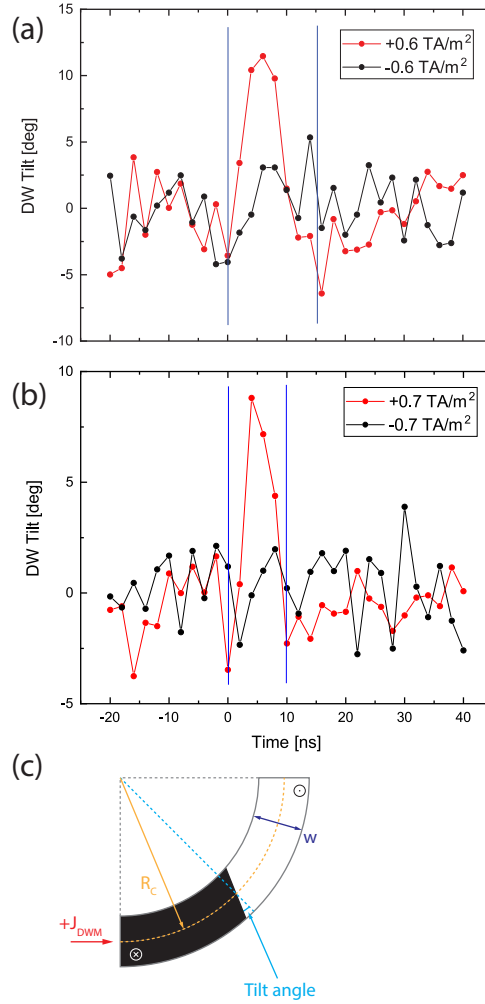
Figure 2. Time traces (2 ns time step) depicting the chiral DW tilting angle during the CIDWM in the Pt/CoB/Ir microwire when applying current pulses of (a) 15 ns, with a spatially averaged current density of 6 \times 10^{11} \text{ A m}^{-2} and of (b) 10 ns, with a spatially averaged current density of 7.2 \times 10^{11} \text{ A m}^{-2} . A clear difference in the DW tilting when inverting the pulse polarity can be observed. The vertical cyan lines mark the time interval during which the current pulse is applied. The convention for the calculation of the DW angle is shown in (c), along with the definition of the radius of curvature R_C and the width w of the Pt/CoB/Ir microwire. The sign convention for the polarity of the CIDWM pulse is depicted in red in (c), where the conventional current direction is indicated. The domain configuration shown in (c) is defined as down-up in this work.
