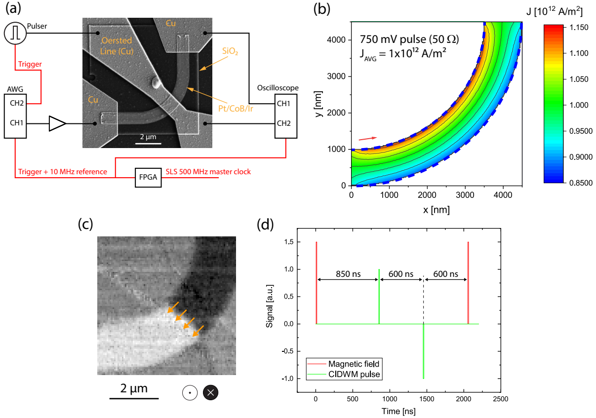
Figure 1. (a) Scanning electron micrograph of one of the 1 \mu\text{m} wide curved Pt/CoB/Ir microwires investigated here. The Oersted line is electrically insulated from the Pt/CoB/Ir microwire by a 100 nm thick SiO 2 film. A schematic overview of the electrical (black) and timing (red) connections is also shown. (b) Finite-element simulation of the current density in the curved microwire upon the injection of a 750 mV pulse (over a termination of 50 \Omega ), resulting in an average current density of 1 \times 10^{12} A m -2 . The non-uniform distribution of the current density in the curved microwire can be observed. The blue dashed line marks the edges of the microwire, while the red arrow indicates the direction of the injected current pulse in the simulation. (c) Quasi-static STXM image of the magnetic configuration of the curved Pt/CoB/Ir microwire after its initialization through the injection of a current pulse across the Oersted line. The legend at the bottom of the image depicts the direction of the magnetization corresponding to the contrast in the image, and the orange arrows in the image depict the chirality of the Néel domain wall by showing the orientation of the in-plane spins in the domain wall. (d) Schematic time trace of the magnetic field and CIDWM pulses employed over one cycle of excitation (about 2 \mu\text{s} ).
