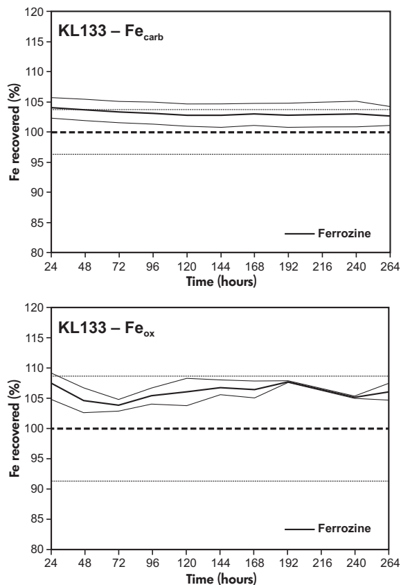
Figure 1. Recovery of Fe for KL133 (solid line \pm 1 s) in the Fe carb and Fe ox fractions, as determined by the spectrophotometric ferrozine method, relative to the mean combined value determined via AAS and ICP-OES (dashed line \pm 1 s).
