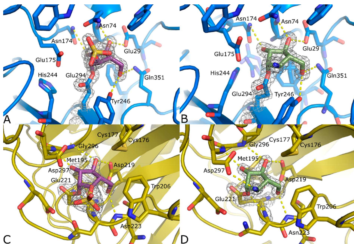
Figure 3. Crystal structures of complexes between inhibitors 2 (B, D, green) and 6 (A, C, purple), and GsGH51 (A, B, blue) and AkAbfB (C, D, yellow). 2F_o - F_c electron density is shown for both the ligand and the catalytic nucleophile as a gray mesh contoured at 2\sigma . The polypeptide is shown in cartoon form with active site residues shown as sticks. Apparent hydrogen bonding interactions are shown as dotted yellow lines.
