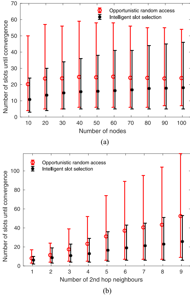
Fig. 4. Joining node's convergence speed. (a) Scalability with the network size. (b) Scalability with the number of 2nd hop neighbors in a 20 node network.
