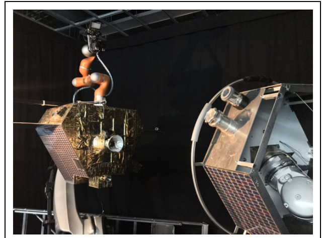
Figure 11. On-orbit simulation (OOS-SIM) facility at DLR.
