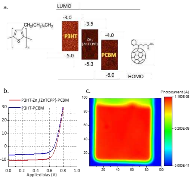
Figure 3 Device performance metrics; a. A representation of the HOMO-LUMO level alignment of the components of the ternary device; b. J-V curve of the best performing devices with and without the MONs; c. High resolution LBIC mapping of the P3HT-MON-PCBM device showing a uniform distribution of current over the entire mapped region, each division on the axes corresponds to the step size = 25microns)
