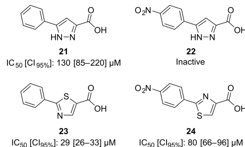
Figure 3. Selected isoxazole ring modifications.
