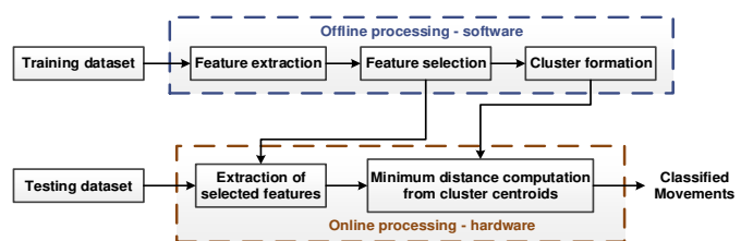
Fig. 1. Processing framework – offline/online processing of the training/testing dataset respectively.
