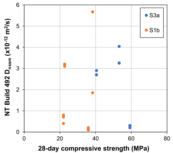
Fig. 6 Correlation between D_{nsm} values determined according to NordTest NT Build 492 by each laboratory (showing individual data points for replicate tests), and the mean 28-day compressive strength measured in the same laboratory, for concretes S3a and S1b
