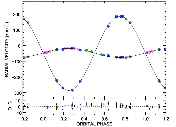
Figure 2. Radial velocity curve of EL CVn. In the top panel, the blue dots represent measurements from HST, green dots the measurements from APO, and published data from Maxted et al. (2014) appear as orchid dots. The errors of the radial velocity measurements are smaller than the dots, and are thus not shown in the top panel. The bottom panel displays the difference between observed and calculated velocities, and the measurement errors are portrayed here. Orbital phase \phi = 0.0 is the epoch when the A-type star reaches inferior conjunction.
