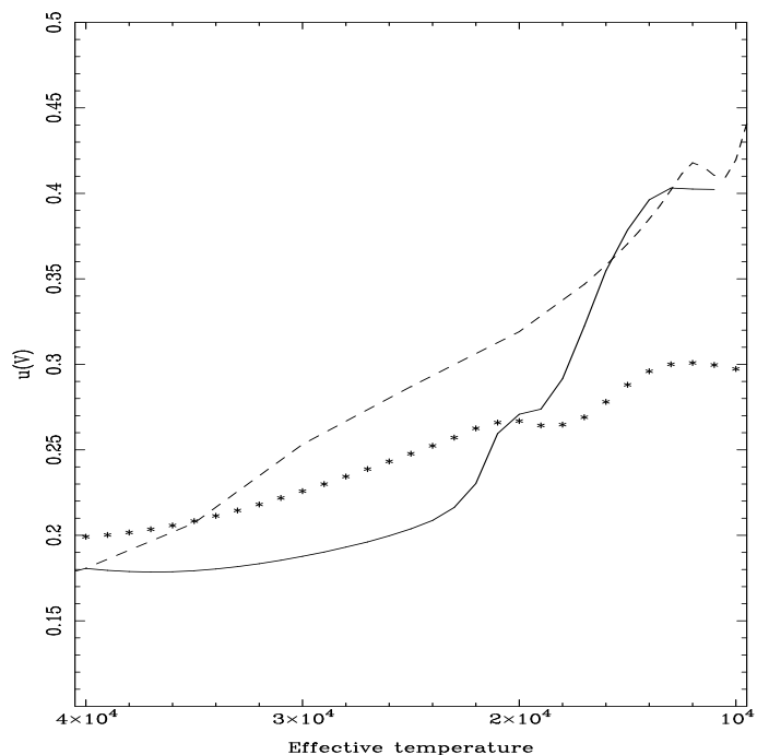
Fig. 6: Linear LDC as a function of the effective temperature for the V passband. Asterisks denote DB models, DBAs (LTE) are represented by the continuous line, and the dashed line indicates DA models. \log g = 7.0 .
