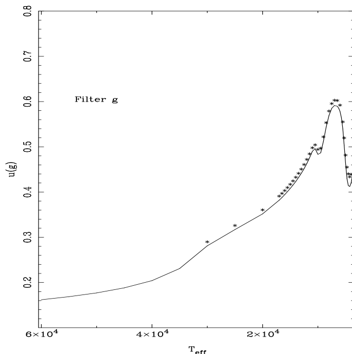
Fig. 7: Comparison between our linear LDCs (continuous line) and those computed by Gianninas et al. (2013), which are denoted by asterisks. DA models, \log g = 6.0 .
