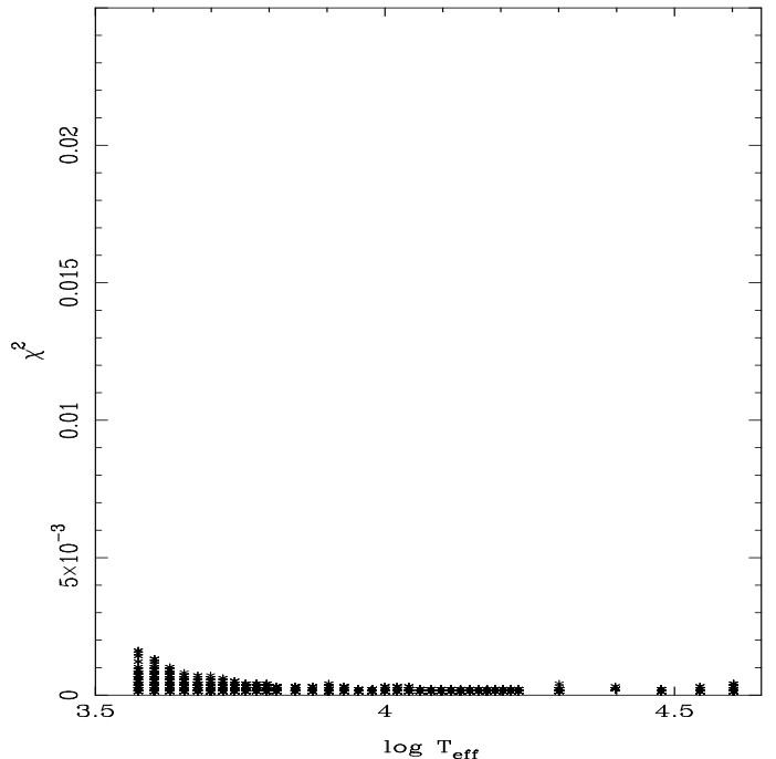
Fig. 3: Merit function \chi^2 for all models of the sample. Four-term law, all Sloan passbands, and DA models (LTE).
