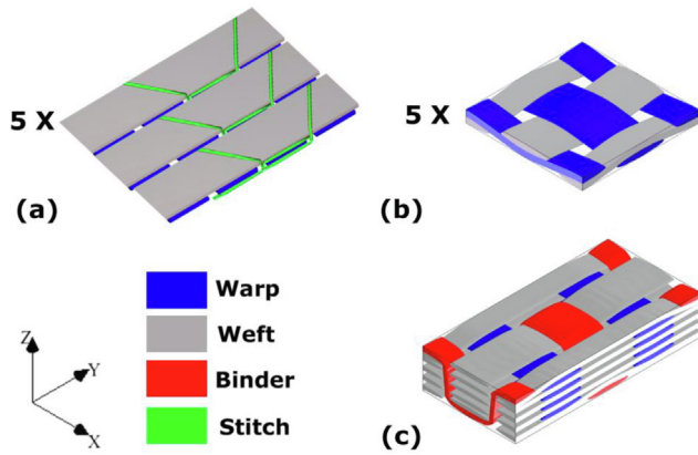
Fig. 1. Schematic of the different types of investigated composites: a) NCF, b) 2D-PW and c) ORT-PW (the warp yarns highlighted in blue, the weft yarns in grey, the through thickness binders in red, and the stitch yarns for the NCF in green) [6]. (For interpretation of the references to color in this figure legend, the reader is referred to the web version of this article.)
