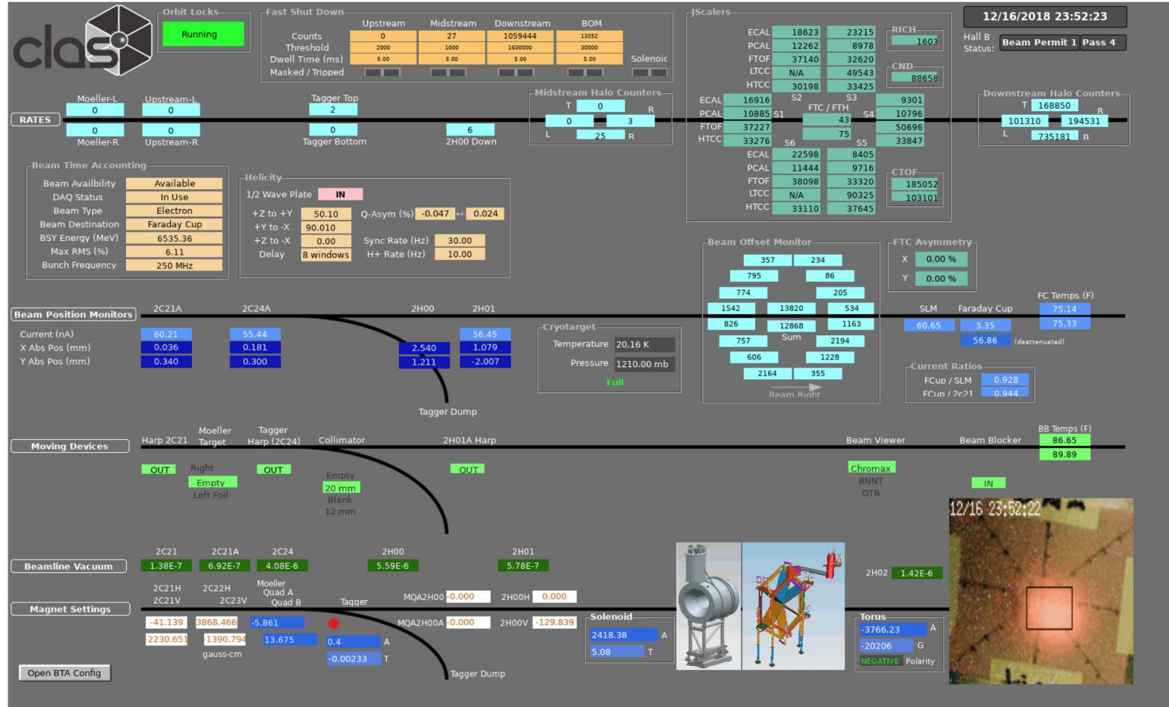
Figure 32: The CLAS12 beamline and detector monitoring systems in Hall B. Top line (left to right) shows the beam halo counters (that typically have zero or single digit rates if the beam quality is good), detector integrated rates in all six sectors, and halo counter rates downstream of the target. Second line: beam position and beam current monitors, status of the cryogenic target, beam offset monitor (16 counters around the beam just upstream of the target), and Faraday cup information. Third line: Devices that can be moved in and out of the beam used for beam viewing and profile measurements, and polarization measurements with Möller scattering. Fourth line: Beamline vacuum conditions, beamline quadrupole settings, CLAS12 torus and solenoid settings, Chromax beam viewer, and beam blocker in front of the Faraday cup.
