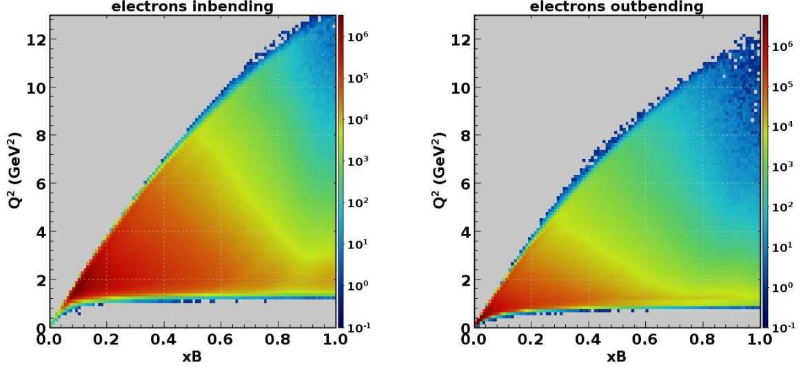
Figure 41: Inclusive ep \rightarrow e'X coverage in Q^2 vs. x_B at a beam energy of 10.6 GeV. The full kinematics is measured simultaneously. The kinematic range is given by elastic scattering kinematics at x_B = 1 , and the small angle acceptance at the Q^2 limit for scattered electrons bending (left) toward the beamline (inbending) or (right) away from the beamline (outbending). The two configurations require opposite directions of currents in the torus magnet coils. Note that the minimal Q^2 is lower for the electron outbending configuration, and that the maximum Q^2 reach is slightly higher for inbending electrons.
