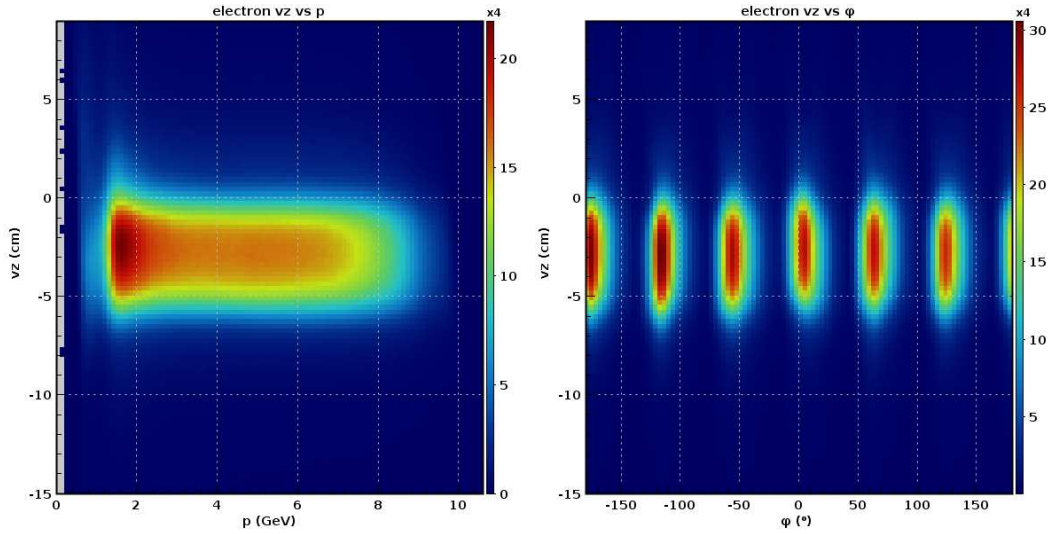
Figure 38: Reconstructed vertex along the beamline vz for electrons in the FD. Left: vz vs. momentum, Right: vz vs. azimuthal angle. The vertical size of the vertex band is consistent with the target length of 5.0 cm.
