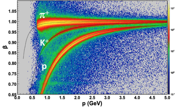
Figure 42: \beta = v/c vs. momentum of positively charged particles detected in the CLAS12 FD. Events were selected to have an electron identified. The charged particle trajectories are reconstructed and their path length and timing from the target to the FTOF (panel-1b layer) are determined. The start time at the target is given by identifying the corresponding beam bucket as time t=0 . The thin black lines show the expected distributions for the respective charged tracks. Particle identification is limited to momenta greater than 0.8 GeV when the torus magnet is energized to maximum current. At reduced torus current the tracking is extended to lower momenta at the expense of momentum resolution.
