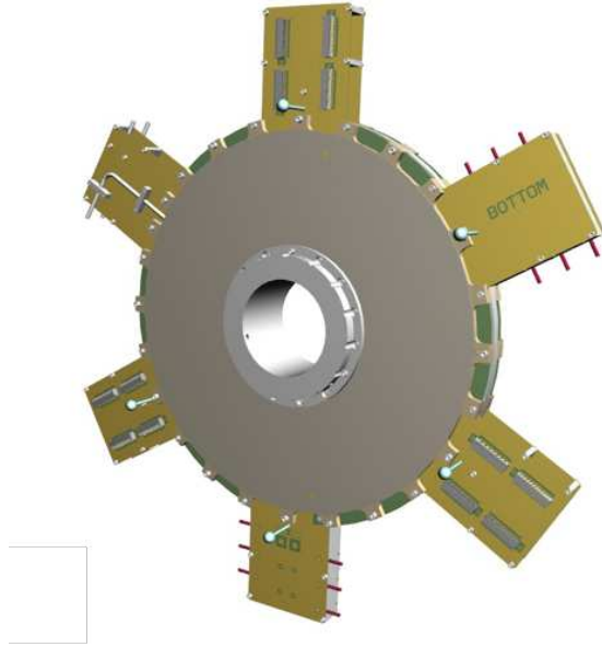
Figure 13: 3D view of the upstream face of the FT-Trk Micromegas tracker equipped with front-end electronics.
