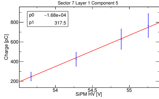
Figure 27: Dependence of the MIP mean position on the SiPM bias voltage for a single hodoscope tile. The dependence is fit to a linear function that is used to select the operating voltage to give an average MIP signal close to the chosen value.
