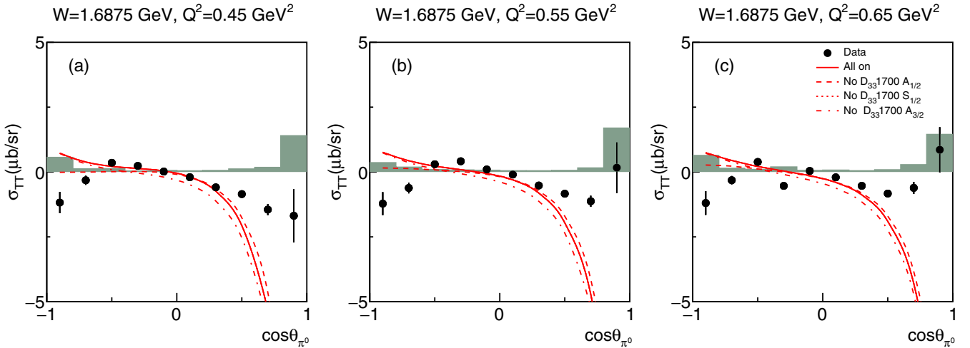
FIG. 24. \sigma_{TT} unpolarized structure function at W = 1.69 GeV and different photon virtualities Q^2 as the functions of \cos(\theta_{\pi_0}^*) c.m. angles in comparison with the JLab/YerPhi model expectations [5] with turned on-off electrocouplings of \Delta(1700)3/2^- resonance: all electrocouplings on (solid lines), A_{1/2} electrocoupling off (dashed lines), S_{1/2} electrocoupling off (dotted lines), and A_{3/2} electrocoupling off (dash-dotted lines). Shaded bands represent systematic uncertainty.
