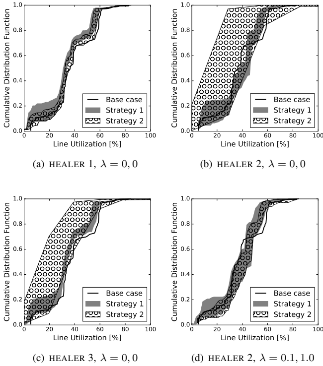
Fig. 7. Lines utilization in case-30 with AC power flow under different healing modes and \lambda values for STRATEGY 1 and STRATEGY 2 respectively.
