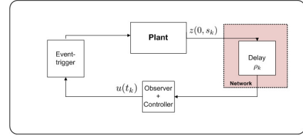
Fig. 2. Network-based control with ET from controller to actuator.
