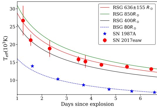
Figure 6. Constraining the progenitor radius of SN 2017eaw based on the cooling of the photospheric temperature in the early phase after the explosion. The red dots are the temperatures inferred from the blackbody fit to the observed UV and optical photometry; while the red curve represents the best fit of the radius. The green and black curves show the upper and lower limits of the estimates of the radius, respectively. The blue stars show the temperature evolution of SN 1987A, and the blue dashed line shows the corresponding best-fitting radius using the theoretical model (Rabinak & Waxman 2011).
