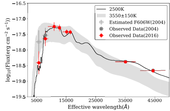
Figure 7. The grey squares and red circles are the SED of the progenitor observed in 2004 and 2016, respectively. The best-fitting result of the observed SED in 2016 with theoretical MARCS stellar spectra indicates the progenitor to be a RSG with effective temperature of 2500K. The open square is the estimated F606W-band result in 2004. And the grey shadow region is the distribution of the SED inferred from the MARCS stellar spectra model with a radius of 636 \pm 155 R_\odot .
