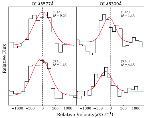
Figure 10. [OI \lambda\lambda 5577, 6300 \text{ \AA} ] sky emission lines. The upper panel shows [OI \lambda\lambda 5577, 6300 \text{ \AA} ] sky emission lines for the t = +1.4 \text{ d} spectrum, while the lower panel indicates the case for the t \sim 3.4 \text{ d} spectrum. The sky emission lines are not corrected for the redshift, and the red lines show the result of Gaussian fit.
