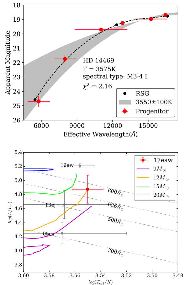
Figure 5. SED of the progenitor star and its location in Hertzsprung–Russell diagram. Upper panel: the SED of the progenitor star compared to that of the Galactic RSGs. The red points represent the SED of the progenitor of SN 2017eaw obtained in 2016, while the black dots represent the ones of RSGs from Milky Way. The black dashed line is yielded by applying a second-order polynomial fit to the values of Galactic RSGs. The grey shadow region represents the distribution inferred from the Galactic RSGs with the temperature ranging from 3450 to 3650 K. Lower panel: the solid lines represent the stellar evolution tracks for 9–20 M_{\odot} , based on the Geneva model (Ekström et al. 2012). The measurements of the progenitors of SN 2005cs (Maund, Smart & Danziger 2005) and SN 2013ej (Fraser et al. 2014) are overplotted for comparison. The dashed straight lines indicate the lines of equal stellar radii.
