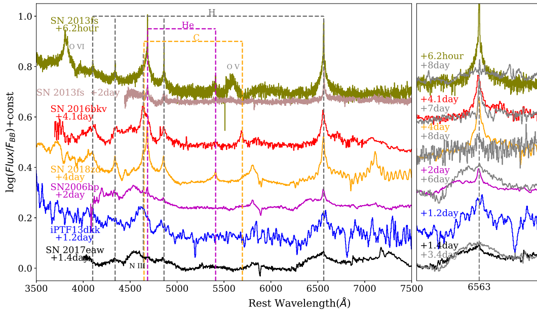
Figure 8. Early time spectroscopy of SN 2017eaw and some comparison SNe II that show clear signatures of CSMs. Left-hand panel: the early spectroscopy of SN 2017eaw, SN 2006bp (Quimby et al. 2007), SN 2013fs (Yaron et al. 2017), iPTF13dkk (Khazov et al. 2016), SN 2016bkv (Nakaoka et al. 2018), and SN 2018zd (from our own data base), covering the wavelength from 3500 to 7500 Å. All the spectra were obtained within 4 d after explosion and have been normalized to the continua and corrected for the host-galaxy redshift. The positions of narrow emission lines of hydrogen, helium, and carbon are marked with dashed lines. Right-hand panel: early-time spectral evolution centering at H \alpha line profile, with the ion-flashed/circumstellar features being initially detected and subsequently having disappeared. The red flux deficiency and blue excess asymmetry feature of H \alpha in the early spectra of SN 2017eaw also disappears in the later spectra (at t \sim +3.4 d) making the line profile symmetric, which is a signature of dust.
