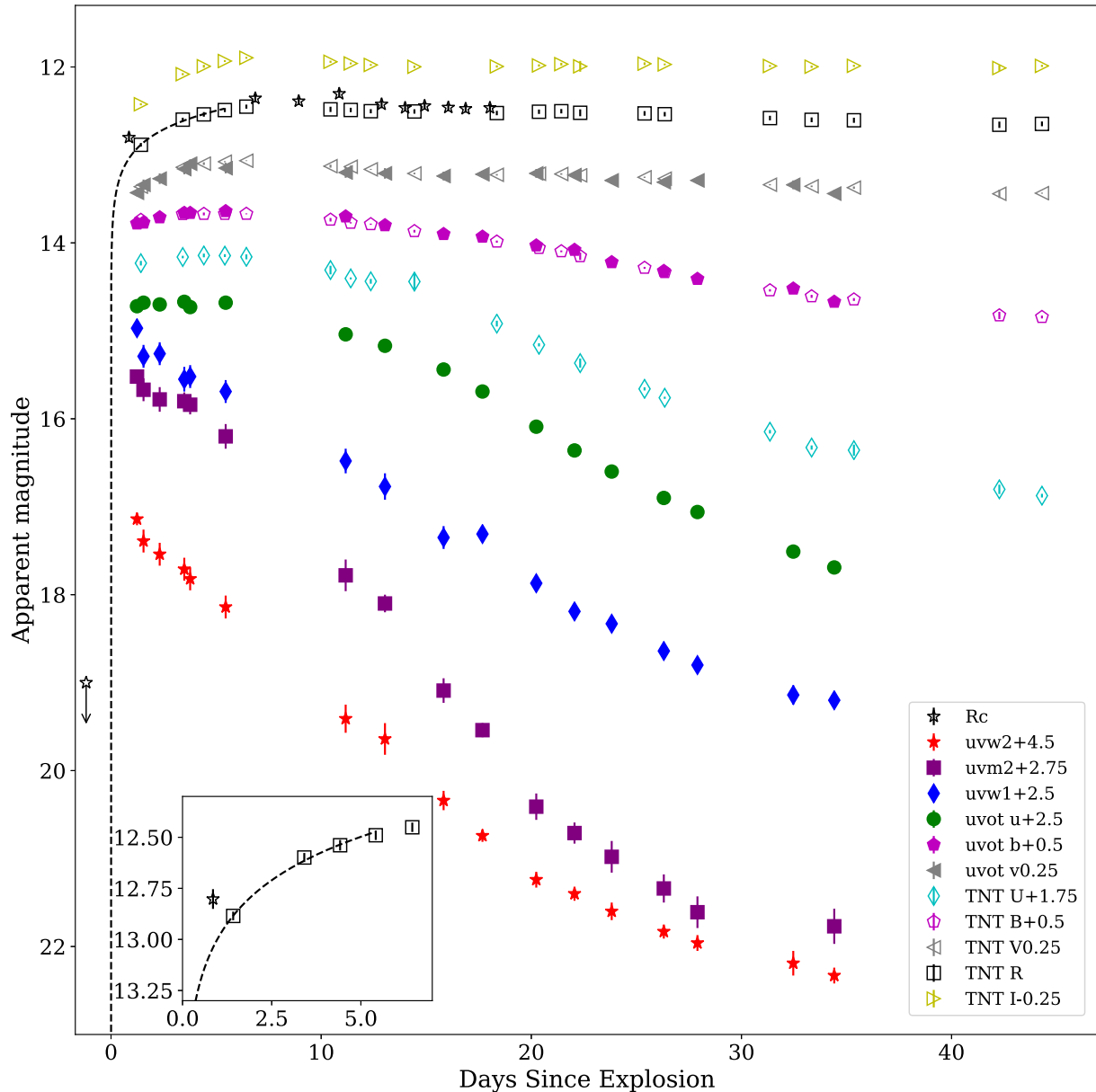
Figure 1. Optical and UV follow-up photometry of SN 2017eaw obtained with the Tsinghua-NAOC 0.8-m telescope (TNT) and the Swift UVOT. The dark dashed lines show the best fit to the R -band data in a form of f \propto (t - t_0)^n , and the first open star represents the last non-detection (unfiltered) from Patrick Wiggins.
