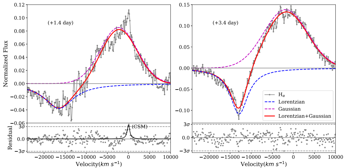
Figure 9. The H \alpha line profile in the earliest two spectra of SN 2017eaw, displayed in a velocity space. Left-hand panel: the H \alpha line profile in t = +1.4 d spectrum. The red curve represents the best-fitting result using a combination of Lorentzian and Gaussian functions, with the blue and magenta curves showing the absorption and emission components of the P-Cygni profile, respectively. Right-hand panel: the same case as in the left-hand panel but for the t = +3.4 d spectrum. The lower panels show the residual of the observed line profile relative to the best-fitting profile; and the narrow emission component in the left-hand panel, due to the CSM, can be fitted by a Lorentzian function with a centre wavelength of 6559.50 \pm 1.31 Å.
