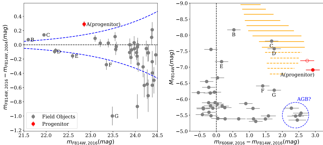
Figure 11. Magnitude and colour variations for the progenitor star of SN 2017eaw and the neighbouring stars at a distance of 200 pc, measured from the HST predisccovery images. Left-hand panel: the F814W-band magnitude variation over the period from 2004 to 2016. The blue dashed lines indicate the 3\sigma limit of the photometric error. The progenitor of SN 2017eaw is represented by symbol ‘A’, and those stars showing larger variations are also labelled with specific symbols. Right-hand panel: the F606W–F814W colour distribution of progenitor and field stars, measured from the HST images taken in 2016. The red open circle represents the colour that the progenitor would have had in 2004 assuming that the observed dimming behaviour is totally due to the obscuration by accumulated dust. The orange solid and dashed lines show the instability region of supergiants for stars in the mass range of 15 < M < 40 M_{\odot} and 10 < M < 15 M_{\odot} , respectively. These regions are obtained by applying the pulsation growth rate to the MIST stellar tracks (Conroy et al. 2018). The objects locating in the dashed circle are likely luminous asymptotic giant branch (AGB) stars according to their luminosity and red colours.
