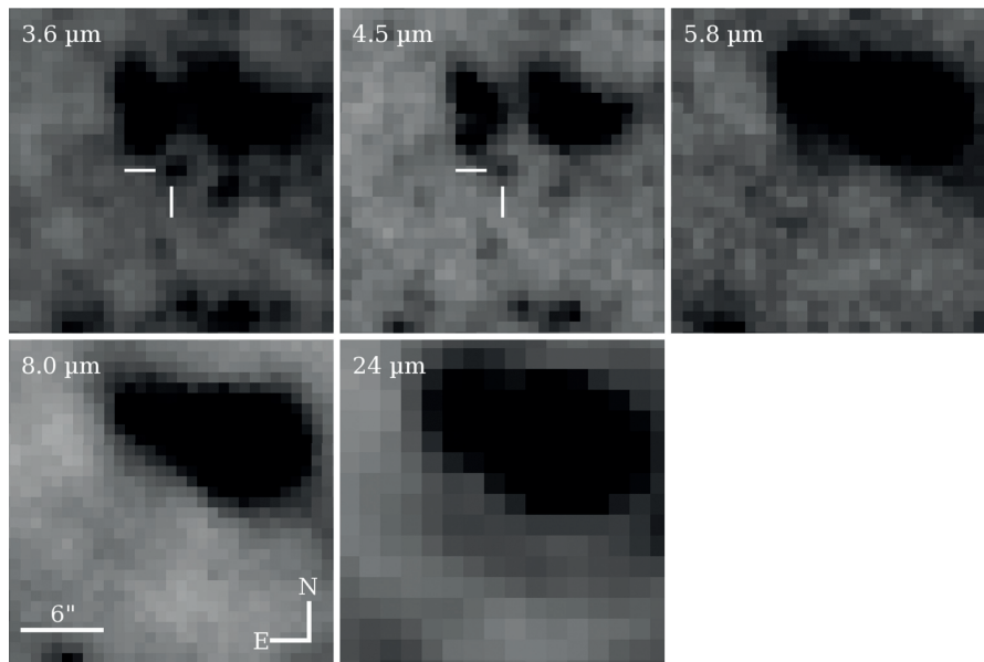
Figure 4. Subsections of pre-explosion Spitzer images centering on the site of the SN. All images are aligned. The white cross hairs in the 3.6 and 4.5 \mu\text{m} images mask the progenitor candidate.
