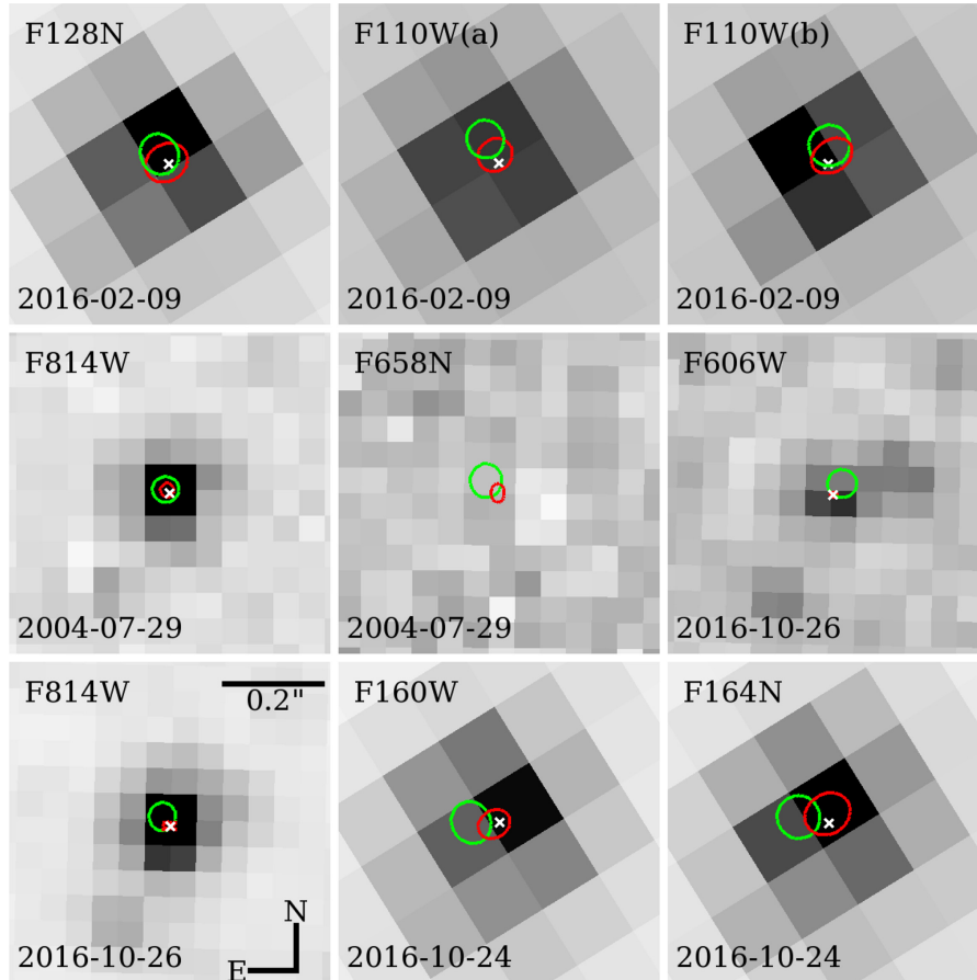
Figure 3. The zoomed-in region of the progenitor site on the HST pre-explosion images. All images are aligned. The white cross marks the measured centre of the possible SN progenitor. The centre of the ellipses shows the transformed SN positions, with the size indicating the uncertainty. Red ellipses show the SN position determined from the post-explosion HST image, while the green ones represent the ones from the post-explosion TNT image. F110W(a): F110W image of icyqf2010_drz.fits; F110W(b): F110W image of icyqe2040_drz.fits.
