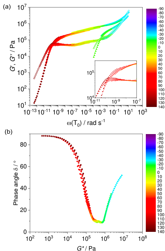
Fig. 3 (a) Rheology master curves for UPy1 ( \Delta ) and Am1 ( \nabla ) shifted using WLF theory. G' solid symbols, G'' open symbols. Colour scale corresponds to the temperature of measurement, in degrees celcius. Inset highlights fanning of the TTS of UPy1 at the terminal region. T_0 = T_g . (b) van Gurp-Palmen plot of UPy1
