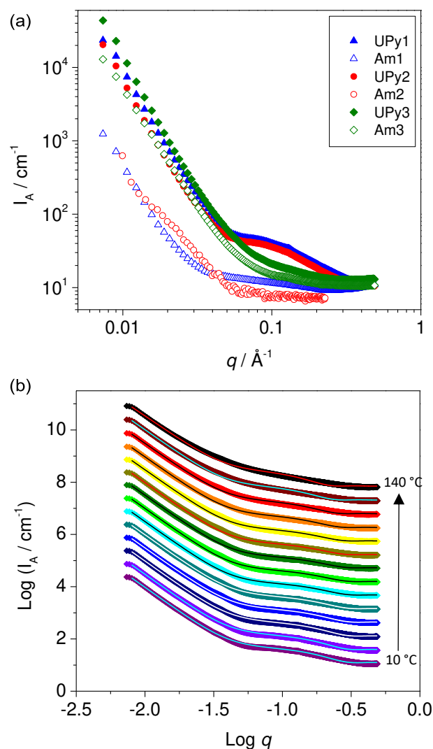
Fig. 6 Small angle X-ray scattering of UPy1, 2 and 3, and Am1, and 3: (a) Scattering intensity as a function of the scattering vector, q ; (b) Fits (lines) of UPy1 at 10–140 °C using combined sphere power law model. Data staggered for clarity.
