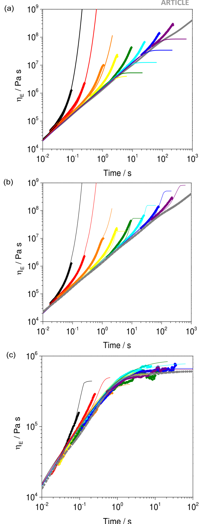
Fig. 7 Extensional viscosity of UPy1 at 25 °C ((a) and (b)) and 80 °C (c), and multi-mode modelling, at strain rates of: 30 (◆), 10 (◆), 3 (◆), 1 (◆), 0.3 (◆), 0.1 (◆), 0.03 (◆) and 0.01 (◆) s -1 . Symbols show experimental data, lines the fits. Linear prediction of viscosity (◆). (a) The model was initially fitted using stretch Rolie-Poly modes around the relaxation times measured from linear oscillatory rheology; (b) Following the initial fit Pom-pom modes were activated for the slowest modes, allowing us to model the strain hardening behaviour across all extension rates; (c) The extensional viscosity of UPy1 was also measured at 80 °C. The model fits at 25 °C in (b) was then shifted using the TTS parameters to 80 °C in (c).
