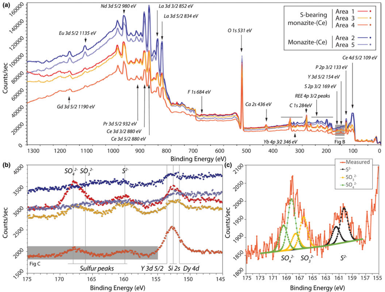
Fig. 5. (a) X-ray photoelectron binding energy spectra of monazite-(Ce) from sites shown in Fig. 3. Note the HREE, S and Ca peaks present in the S-bearing monazite-(Ce). (b) Narrow scan of the Dy, Si, Y and S peaks. (c) Narrow scan of the S 2p binding energy peak indicating sulfur present as sulfite, sulfate and sulfide structurally bound in monazite-(Ce). Binding-energy peak positions from ThermoScientific, xpsimplified.com (accessed 2017), NIST XPS database (accessed 2017), Yu et al. , (1990), Vasquez (1991) and Abraham and Chaudhri (1986).
