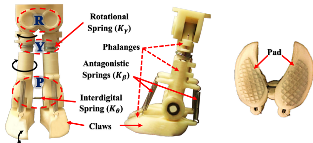
Fig. 5. Abstraction of the goat hoof. It comprises (a) the variable compliance joints fetlock joint (R), pastern joint (Y), coffin joint (P), phalanges (with their respective rotation illustrated with the black arrows), claws, and springs changed during the experiments, and (b) pad.
