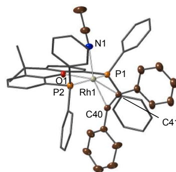
Fig. 4. Solid-state structure of the cationic portion of complex 4 . Selected bond lengths (Å) and angles ( ^\circ ): Rh1–P1, 2.2917(6); Rh1–P2, 2.2922(6); Rh1–O1, 2.2754(15); Rh1–N1, 2.152(2); Rh1–C40, 2.072(2); Rh1–C41, 2.050(2); C40–C41, 1.271(4); O1–Rh1–N1, 80.99(7); P1–Rh1–P2, 161.76(2).
