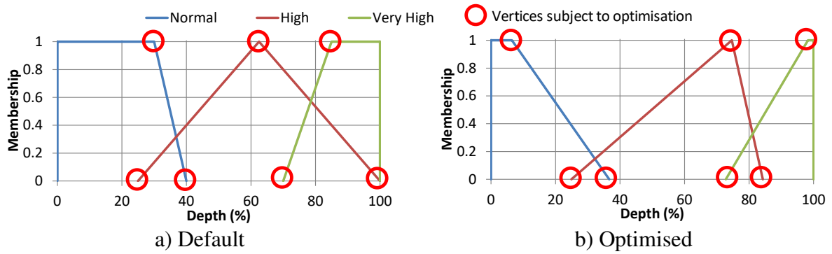
Figure 3: Example input Membership Functions for level at flood location
