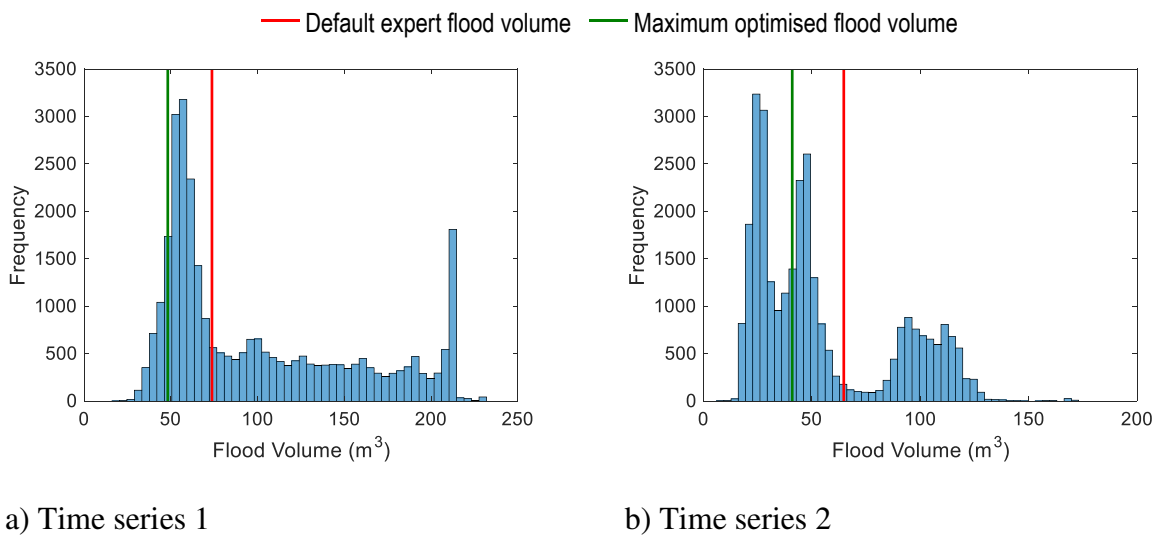
Figure 5: Histogram of Monte Carlo runs for 1 minute time step, decimal MFs.
