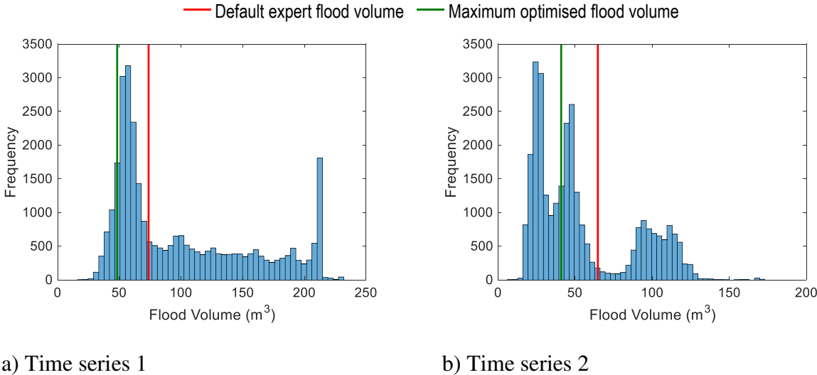
Figure 5: Histogram of Monte Carlo runs for 1 minute time step, decimal MFs.
