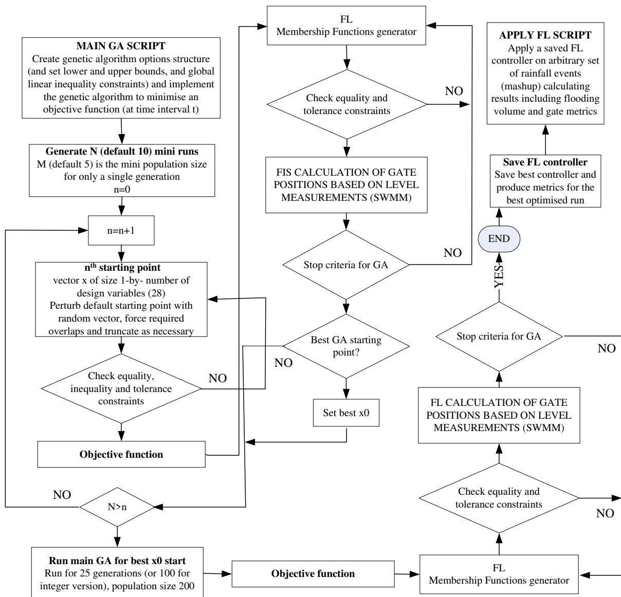
Figure 4: Flow diagram for GA optimisation module
