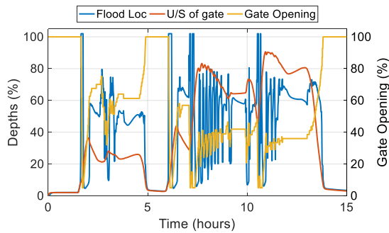
c) Optimised, Pseudo-Random initialisation strategy, RNG shuffled, flood volume 22.62 m 3 , gate # 239, gate dist. 3.44 m.
