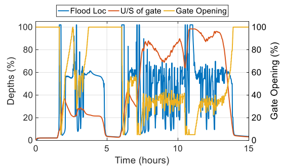
d) Optimised, random initialisation strategy, RNG shuffled, flood volume 21.42 m 3 , gate # 381, gate dist. 5.27 m.
