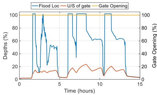
a) Gate inactive (control), flood volume 128.2 m 3 .
