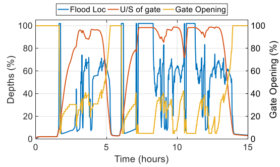
b) Default expert, un-optimised, flood volume 73.7 m 3 , gate # 268, gate dist. 3.52 m.
