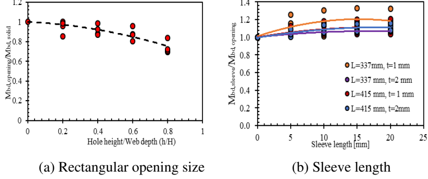
Figure 7: Effect of sleeve length and web opening size on the bending capacity
