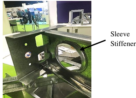
Figure 1: LCB with sleeve stiffened web openings
