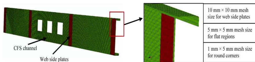
Figure 3: Mesh refinements of FE models
