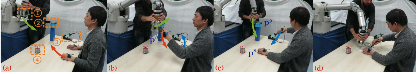
Fig. 4. The collaborative hand task in the soldering environment with the Barrett WAM robot. (a) shows the initial state of the user hands and the robot end-effector (i.e., the collaborative hand in this experiment). ①–④ separately correspond to the circuit board (held by the robot), magnifying glass, soldering iron and solder. (b) corresponds to the handover of the circuit board. (c) shows the robot grasping of the magnifying glass. (d) depicts the final scenario of the soldering task using both of the user hands and the robot end-effector. Red, blue and green arrows depict the movement directions of the user left hand, right hand and the robot end-effector, respectively.
