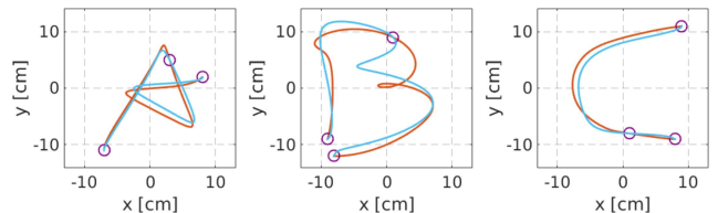
Fig. 2. Comparison of trajectory modulations by using KMP (red curves) and ProMP (blue curves), where circles denote desired points
