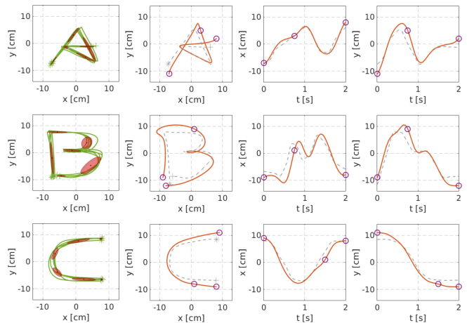
Fig. 1. Trajectory modulations using KMP on hand-written letters. First column shows the demonstrations of various hand-written letters and their corresponding GMM modeling, where the red solid ellipses represent Gaussian components. Second–fourth columns show the adapted trajectories (red solid lines) with different desired points (purple circles). The dashed gray curves depict the original reference trajectories, obtained as explained in Section II-A.
