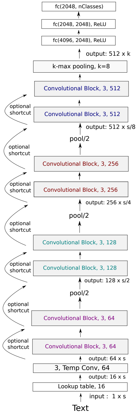
Figure 1: VDCNN architecture.
