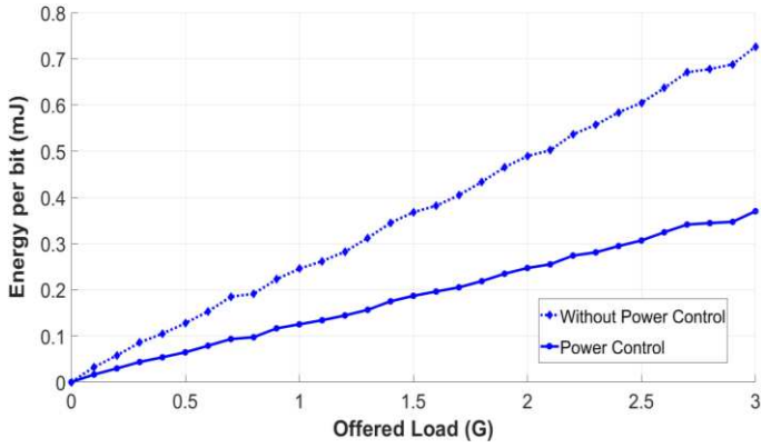
Figure 3. The reduction of required transmission energy per bit due to the proposed power control scheme.
