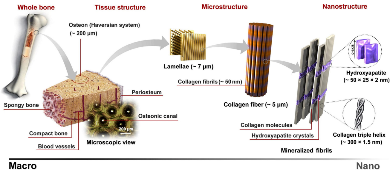
FIGURE 2: This figure illustrates the porous structure of bone at multiple length scales (from macro to nanoscale). If we magnify a section of cortical bone we see that it consists of osteons which, in turn, are made of lamella with osteocytes interspersed. Each lamella consists of collagen fibers which in turn are made up of fibrils. These are composed of collagen molecules with calcium apatite-like inorganic crystals interspersed as shown here and the basic building block is the collagen triple helix. Reprinted from "Synthesis methods for nanosized hydroxyapatite with diverse structures," Sadat-Shojai et al, Acta Biomater 2013;9:7591–6721 with permission from Elsevier (License No. 4661520035459).
