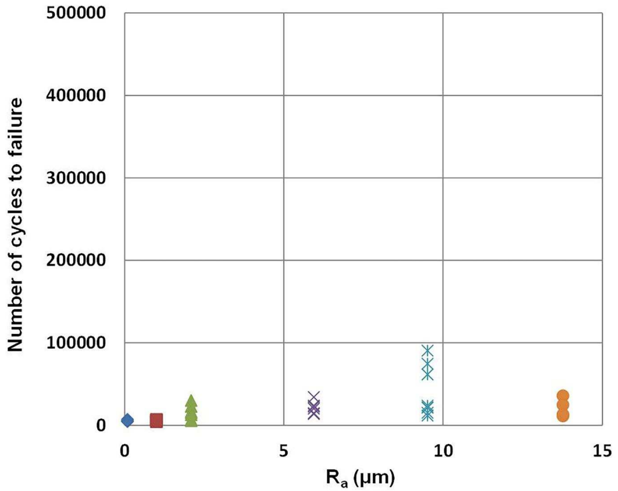
Fig. 9. Number of fretting cycles to failure (100 mΩ failure criterion) as a function of bottom coupon surface roughness. Displacement amplitude applied \pm 20 μm.
