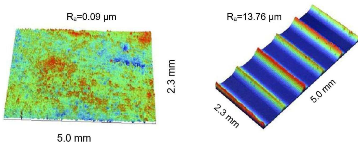
Fig. 3. Left: Surface morphology of a sample polished with 1200 grade sand paper and mirror finished with a diamond paste. Right: milled sample. See Fig. 4 for detailed metrological values.
