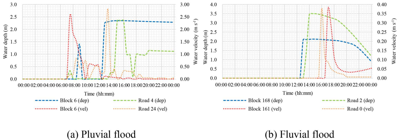
Figure 10. Changes in the surface water depths and velocities for eight severely flooded areas. The “dep” indicates water depth, and “vel” indicates water velocity.
