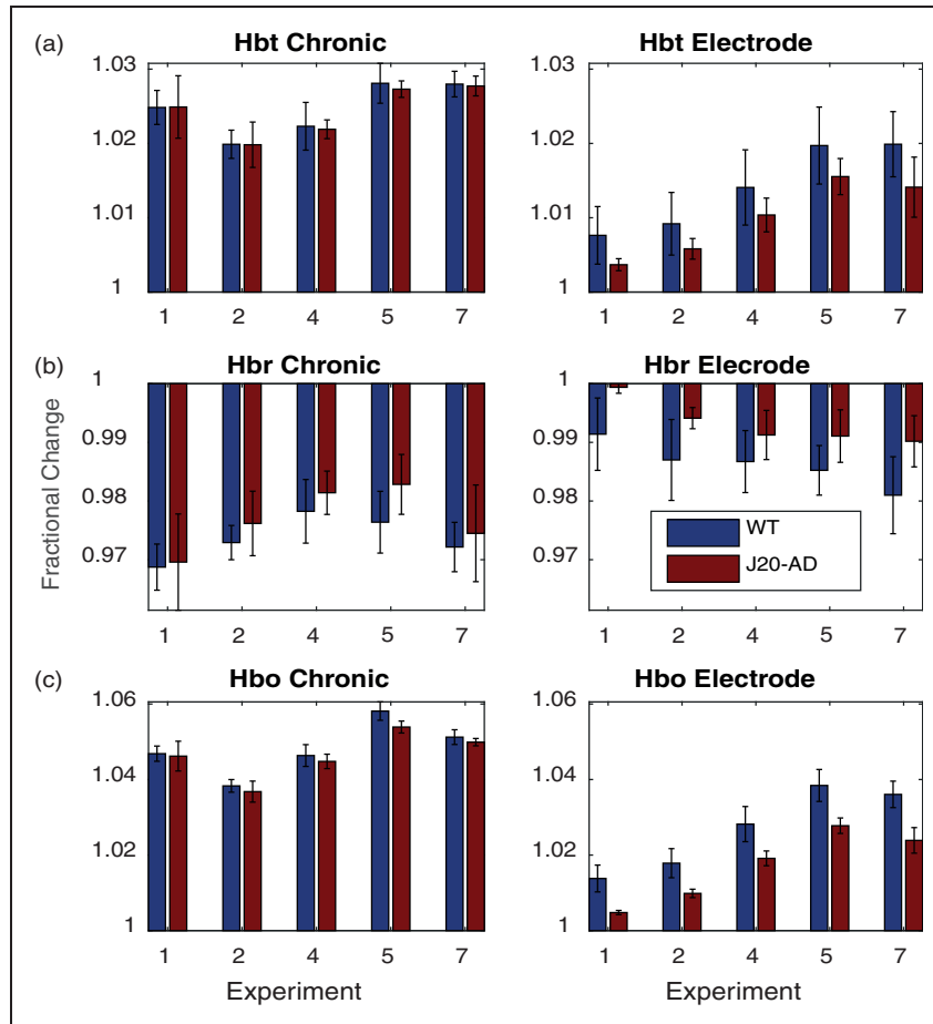
Figure 4. Average magnitude of fractional hemodynamic response for both chronic (left hand side) and acute session (right hand side) stimulation experiments. (a) Hbt (b) Hbr and (c) Hbo. Error bars =standard deviation.
