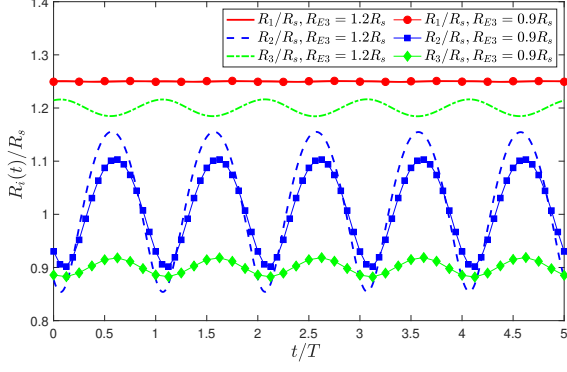
Figure 7: R_i(t) for two different R_{E3} , with R_{E1} = 1.25R_s , R_{E2} = R_s , D_{23} = 10(R_{E2} + R_{E3}) , and p_a = 0.01p_{\text{atm}} . D_{12} = 100R_s .
